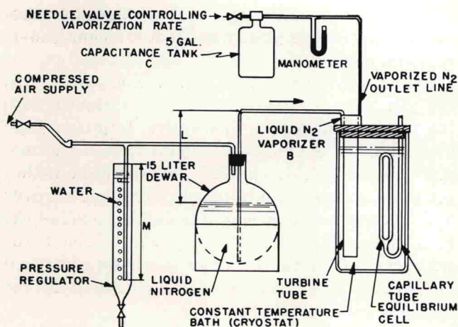
Fig. 10.—Low-Temperature Bath Cooling System
